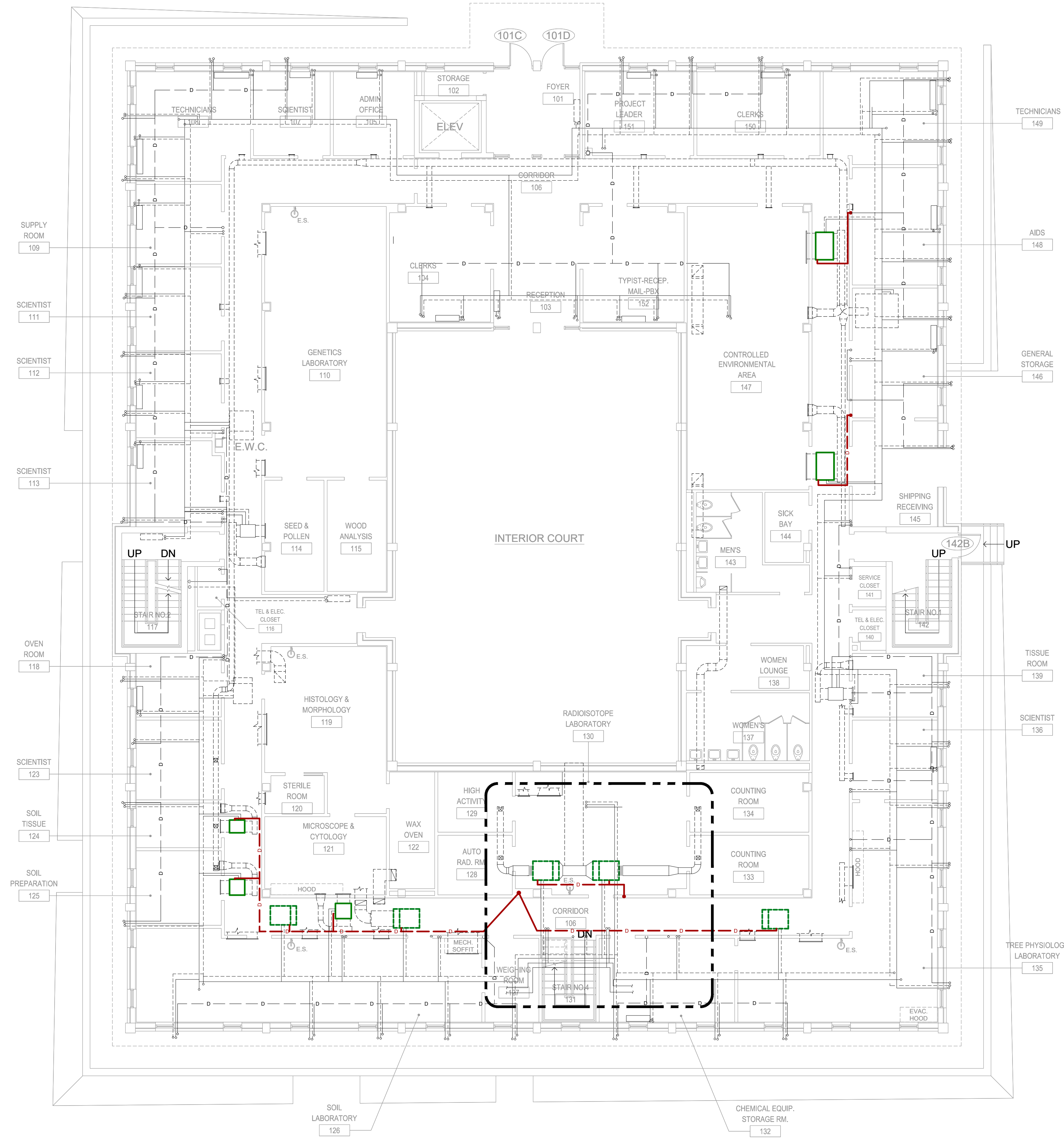
1 NORTH BUILDING FIRST FLOOR, HVAC EXISTING M-152 SCALE: 1/8" = 1'-0"
