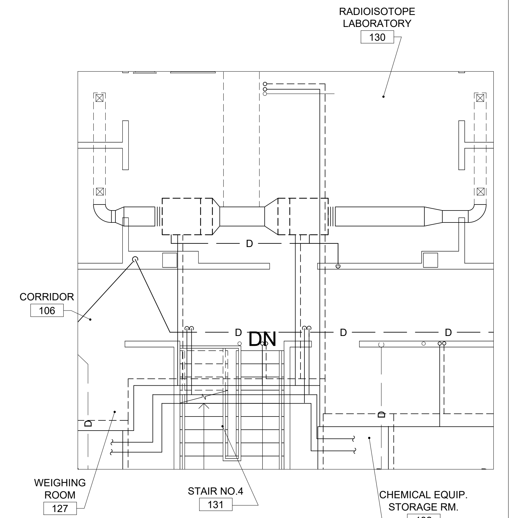
2 ENLARGED FIRST FLOOR PART PLAN M-152 SCALE: 1/4" = 1'-0"
