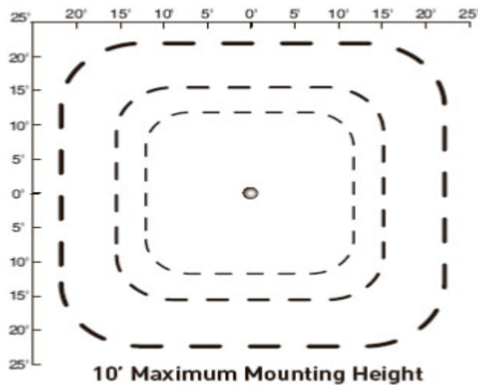
Figure B-8. Coverage Pattern of Ultrasonic Sensor
