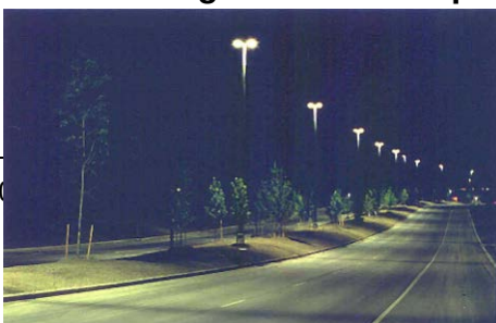
Figure D-3. Examples of IES fully shielded luminaires
