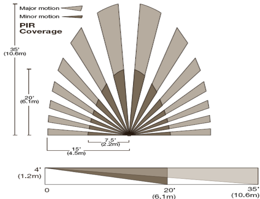
Figure B-7. Coverage Pattern of PIR Sensor
